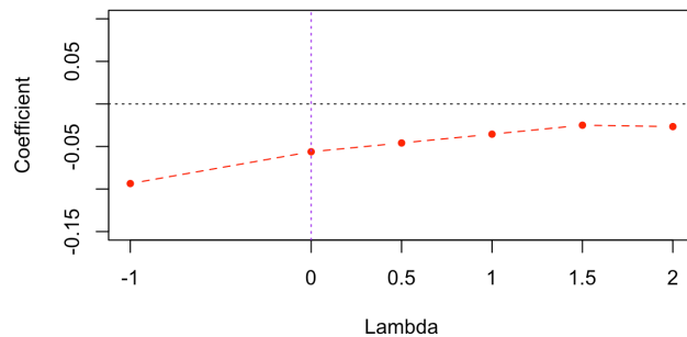
Non- Differential Misclassification
